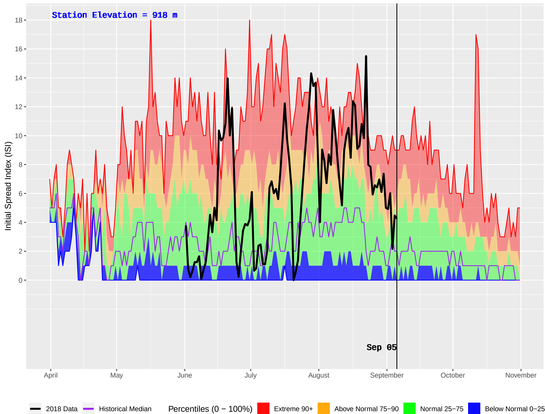
AUGIER LAKE (167) : Historical (1984–2016) and Current (2018) Daily Initial Spread Index (ISI)
