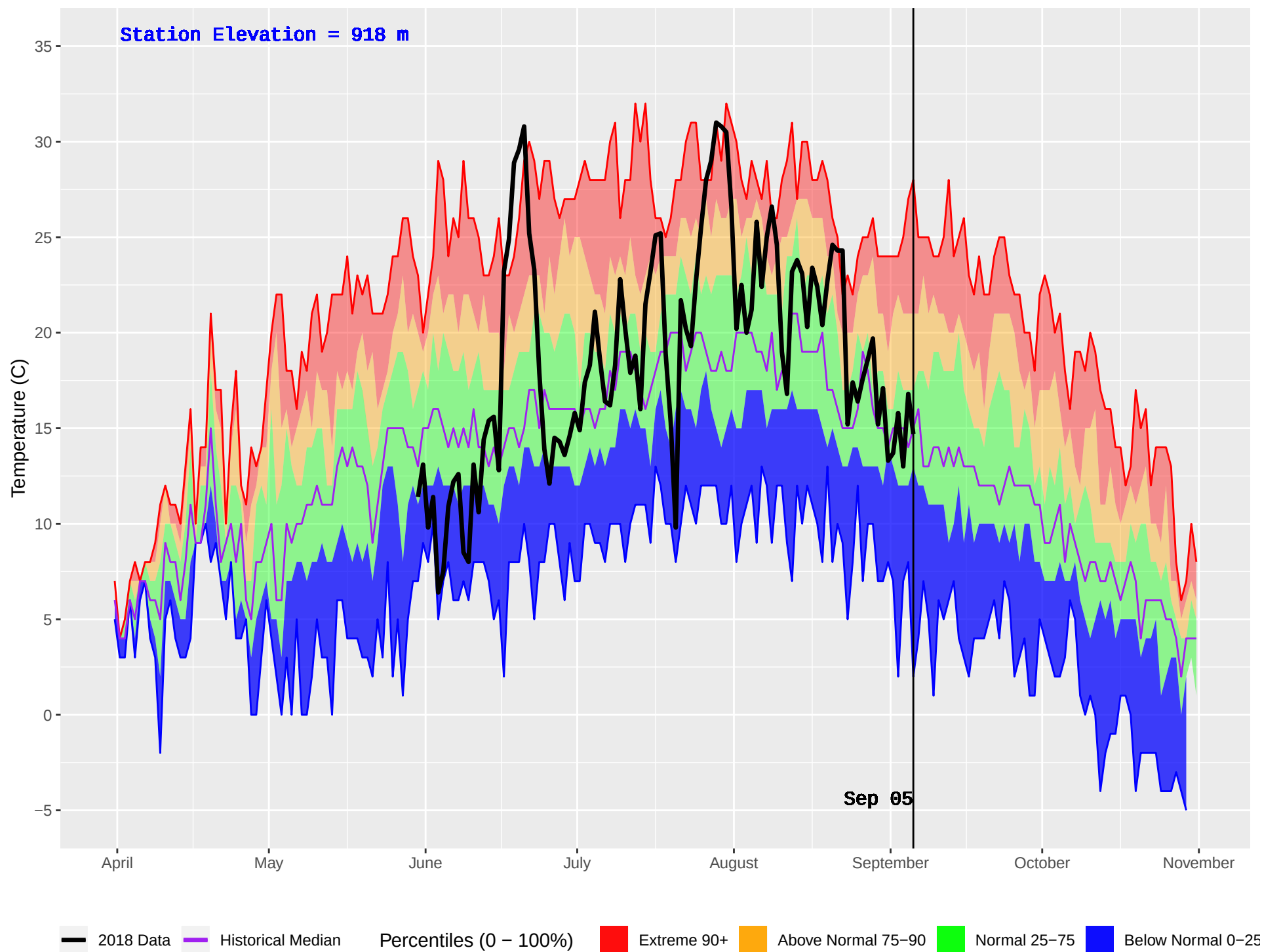
AUGIER LAKE (167) : Historical (1984–2016) and Current (2018) Daily Temperature
