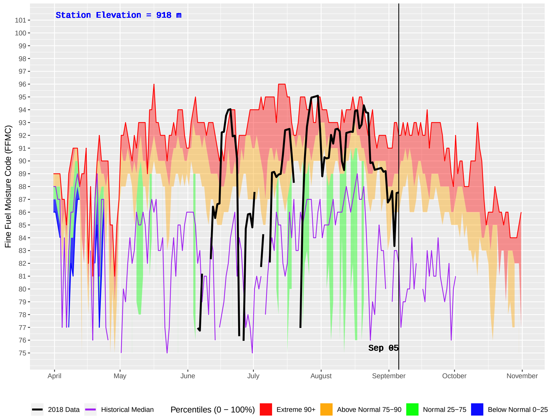
AUGIER LAKE (167) : Historical (1984–2016) and Current (2018) Daily Fine Fuel Moisture Code (FFMC)
