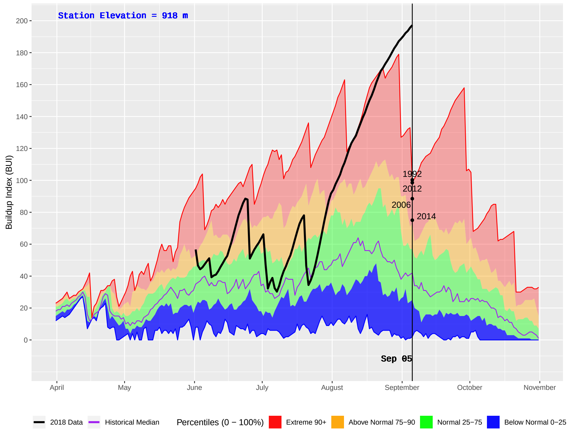
AUGIER LAKE (167) : Historical (1984–2016) and Current (2018) Daily Buildup Index (BUI)
