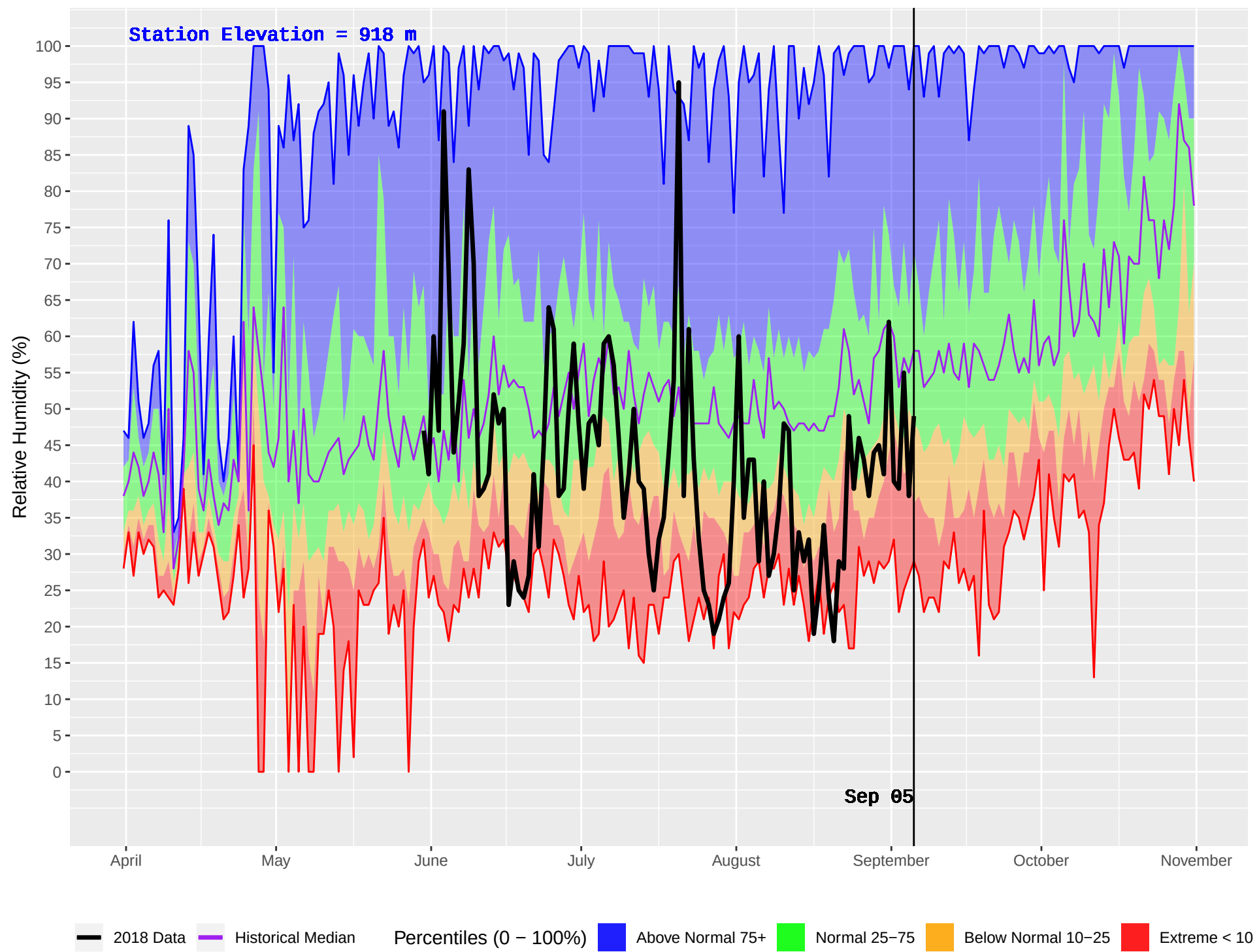
AUGIER LAKE (167) : Historical (1984–2016) and Current (2018) Daily Relative Humidity
