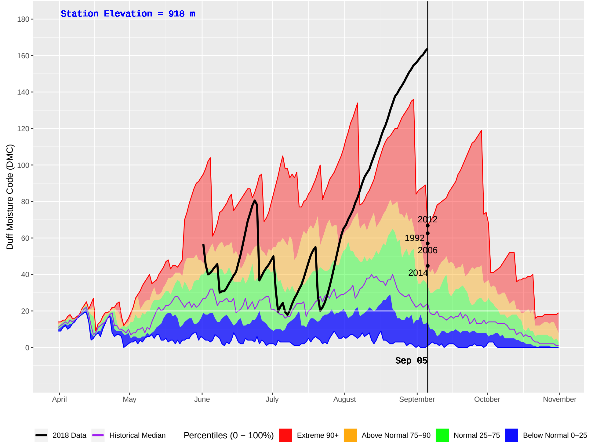
AUGIER LAKE (167) : Historical (1984–2016) and Current (2018) Daily Duff Moisture Code (DMC)
