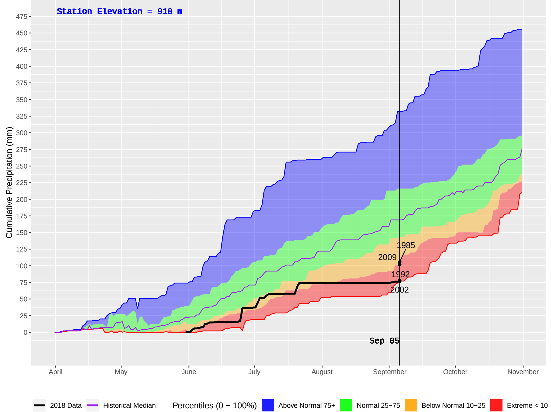
AUGIER LAKE (167) : Historical (1984–2016) and Current (2018) Daily Cumulative Precipitation
